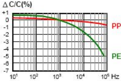
Frequency Characteristics
